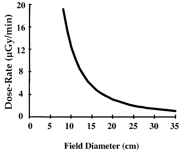
Figure 2. Computed dose rate for a constant DAP reading as a function of field diameter.
