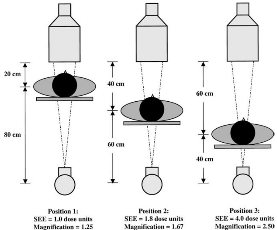
Figure 4. Effect of geometric magnification on entrance skin dose. With fixed source-to-image receptor distance, both magnification and skin entrance exposure ( SEE ) increase as the patient is moved closer to the x-ray source.
