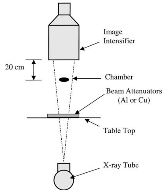
Figure 1. Setup for measuring receptor entrance exposure rates. Constant beam attenuators (aluminum or copper) are placed on the table top or the surface of the collimator (11,12). Measurements are performed by placing the ionization chamber 20 cm from the surface of the image receptor with the grid removed.
