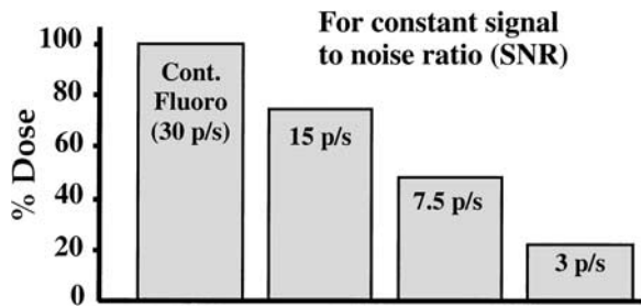
Figure 6. Effect of pulsed fluoroscopy on entrance skin dose. For example, by switching from continuous fluoroscopy ( Cont Fluoro ) mode to 15 pulses per second, dose savings of nearly 22% are achieved (34).
